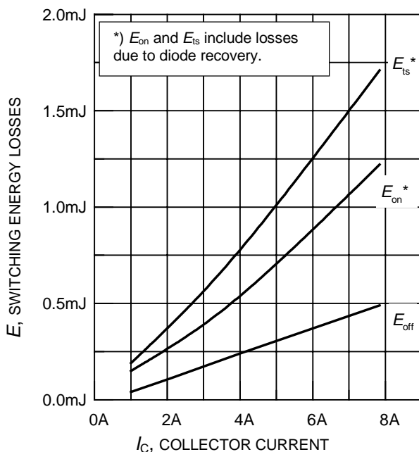
Figure 13. Typical switching energy losses as a function of collector current (inductive load, T_j = 150^\circ\text{C} , V_{CE} = 800\text{V} , V_{GE} = +15\text{V}/0\text{V} , R_G = 91\ \Omega , dynamic test circuit in Fig.E )
